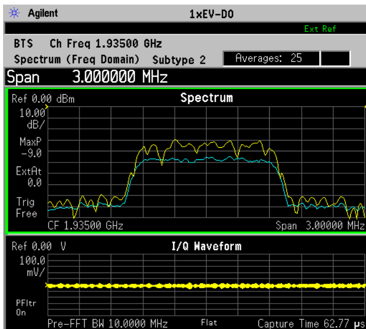
Figure 2-51 Spectrum Measurement - Spectrum and I/Q Waveform (Default View)
