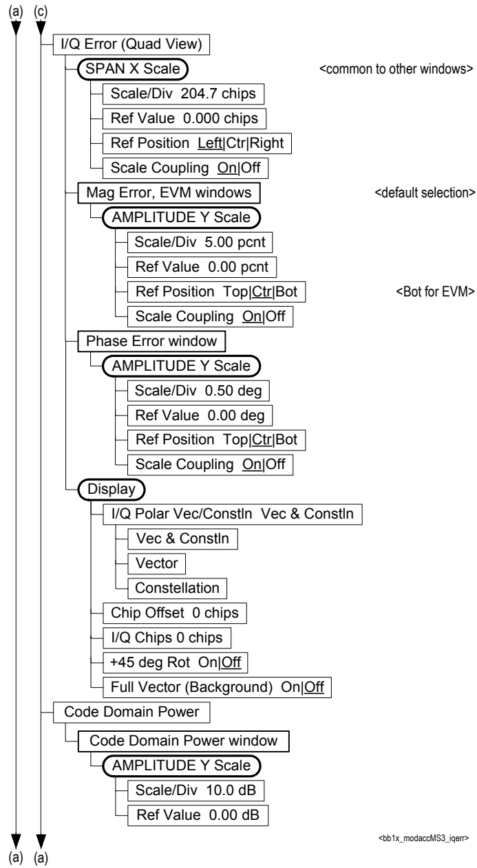
Figure 6-27 Reverse Link Mod Accuracy Measurement Key Flow (3 of 4)
