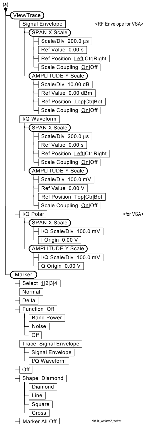
Figure 6-37 Waveform (Time Domain) Measurement Key Flow (2 of 2)
