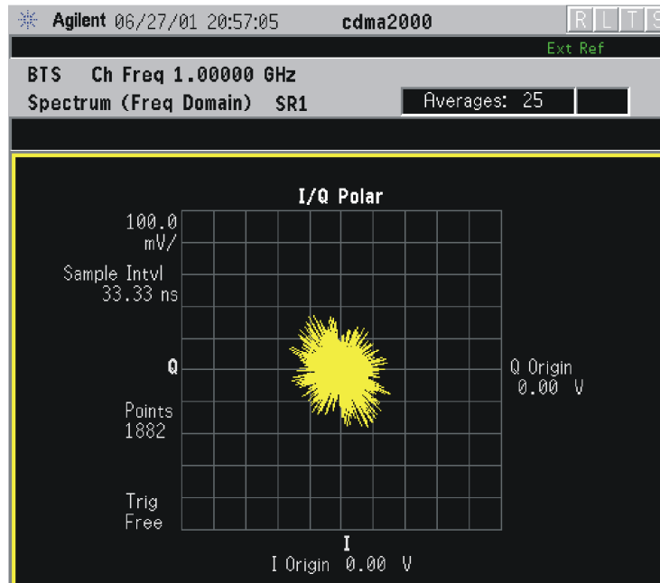
Figure 2-60 Spectrum Measurement - I/Q Polar View (for E4406A)
