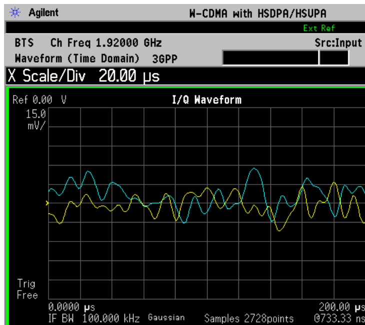
Figure 2-61 Spectrum Measurement - I/Q Polar View (for E4406A)
