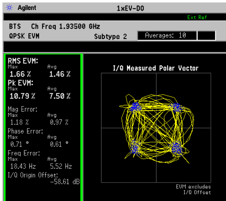
Figure 3-23 QPSK EVM Measurement - I/Q Polar Vector View
