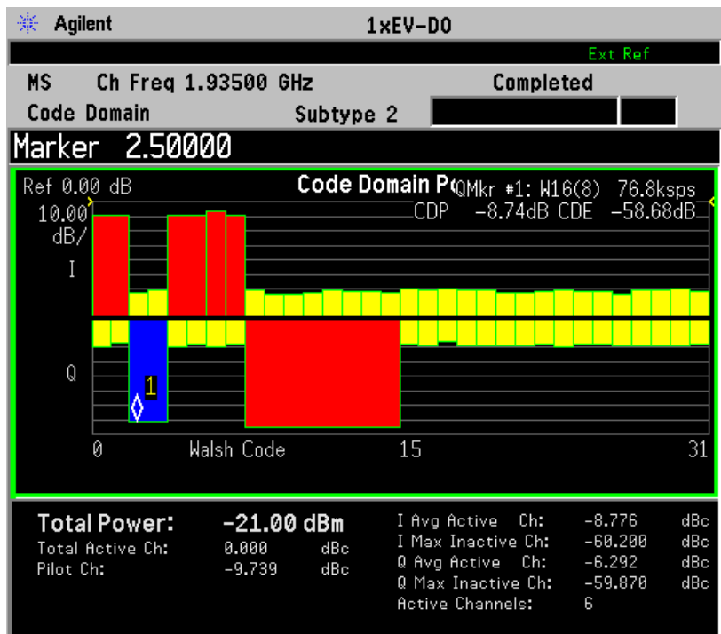
Figure 2-17 Reverse Link Code Domain Result - Code Domain Power Graph View Displayed in Bit Reverse
