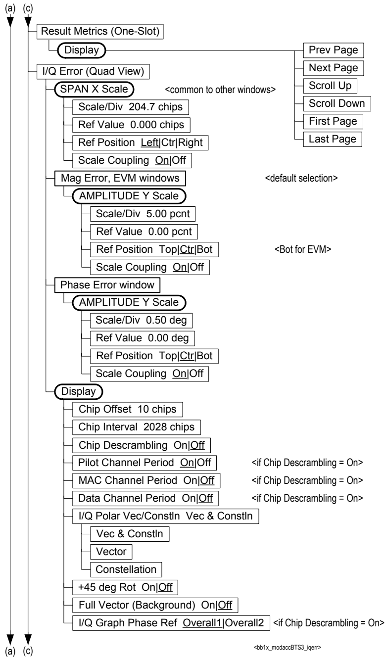
Figure 6-13 Forward Link Mod Accuracy Measurement Key Flow (4 of 6)
