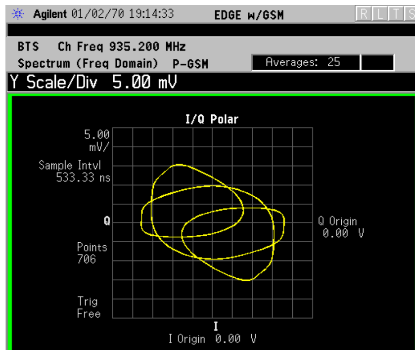
Figure 3-32 Spectrum Measurement - I/Q Polar View (for E4406A)
