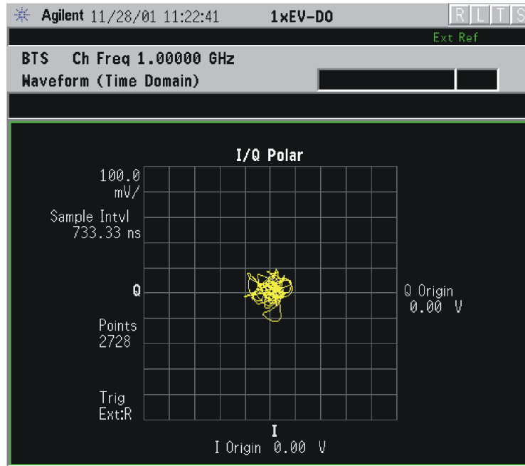
Figure 2-74 Waveform Measurement - I/Q Polar View
