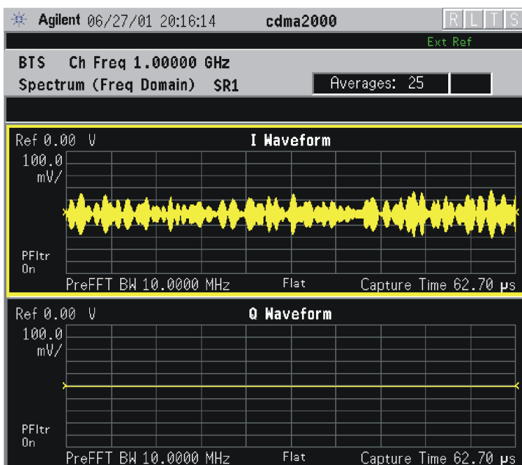
Figure 2-55 Spectrum Measurement - I and Q Waveform View (for E4406A)
