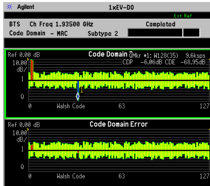
Figure 3-5 Code Domain Measurement - CDP Graph and CDE Graph View
