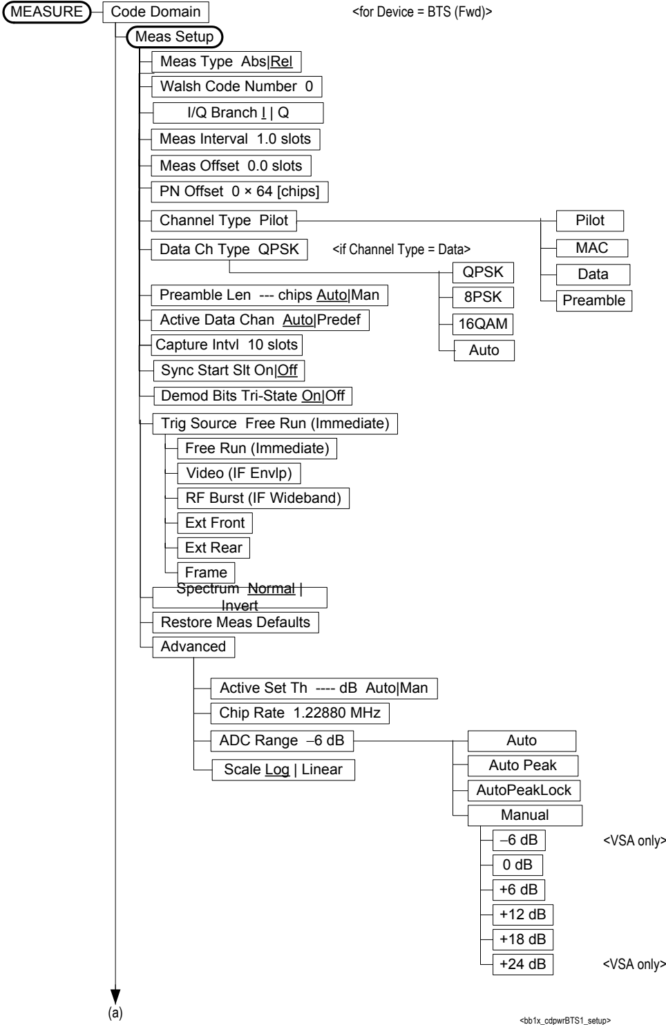
Figure 6-6 Forward Link Code Domain Measurement Key Flow (1 of 4)
