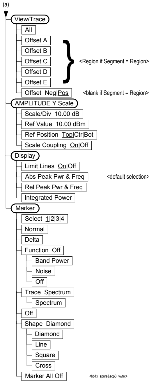
Figure 6-35 Spurious Emissions & ACP Measurement key Flow (3 of 3)
