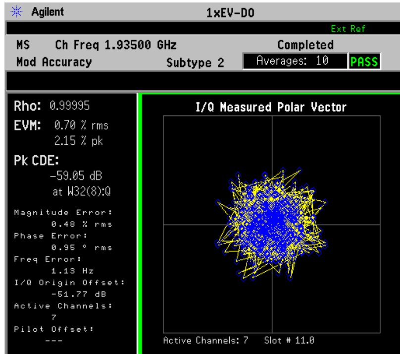
Figure 2-35 Reverse Link Modulation Accuracy Measurement Result - Measured Polar Vector Graph (Default) View
