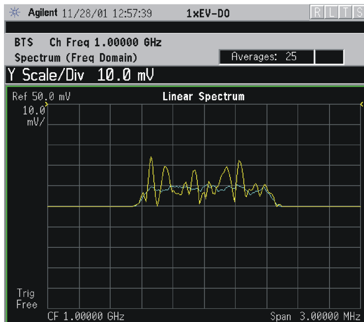
Figure 2-52 Spectrum Measurement - Linear Spectrum View (for E4406A)
