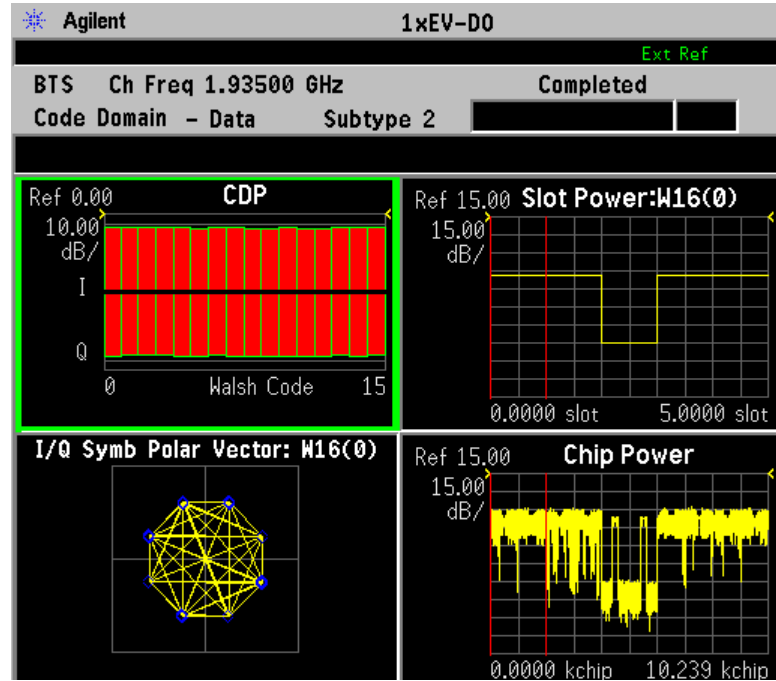
Figure 3-6 Code Domain Measurement - Code Domain Quad View
