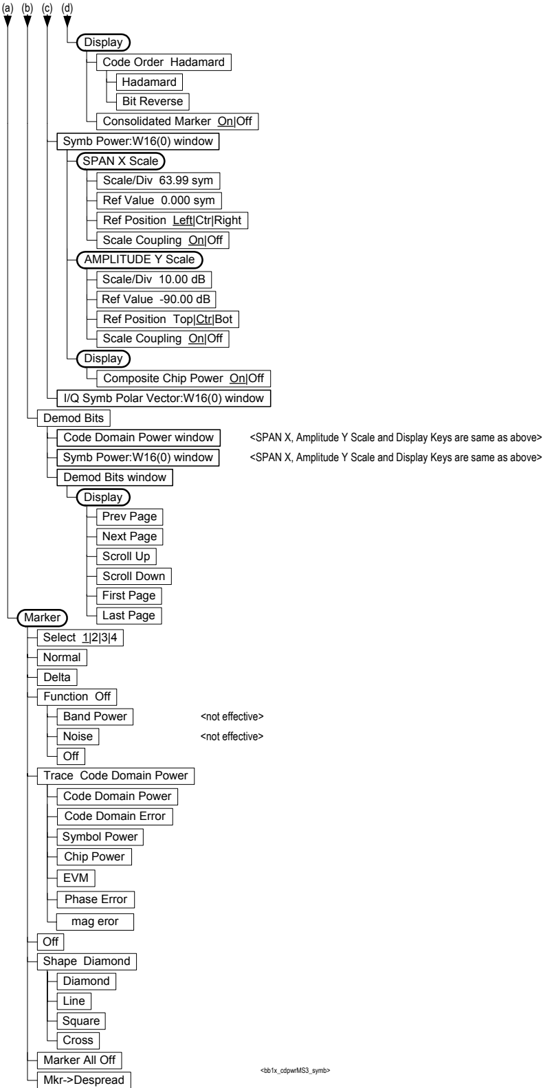
Figure 6-24 Reverse Link Code Domain Measurement Key Flow (3 of 3)
