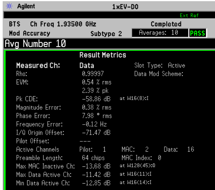
Figure 3-14 Forward Link Modulation Accuracy - Result Metrics (One-Slot) View
