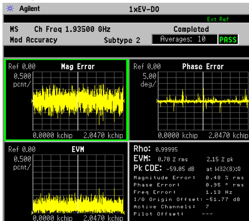
Figure 2-37 Reverse Link Modulation Accuracy Measurement Result - I/Q Error Quad View
