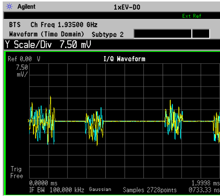
Figure 2-69 Waveform Measurement - I/Q Waveform View
