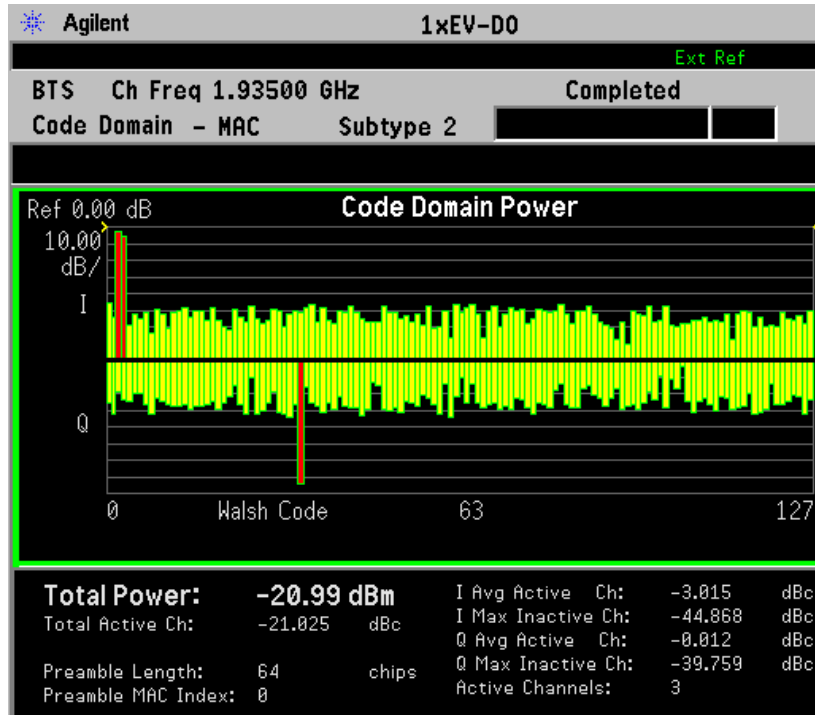
Figure 2-8 Forward Link Code Domain Result - MAC Channels Subtype 2
