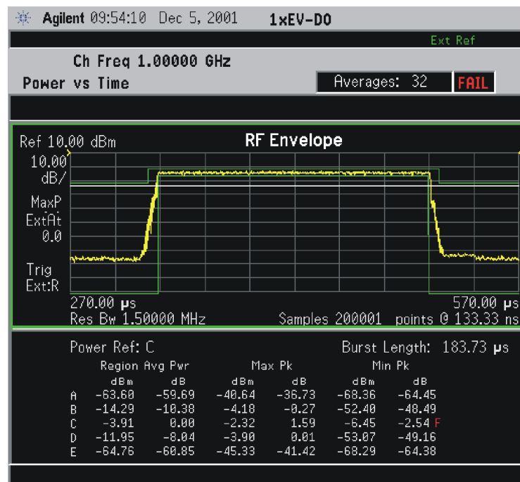
Figure 3-22 Power vs. Time Measurement - Rise & Fall View
