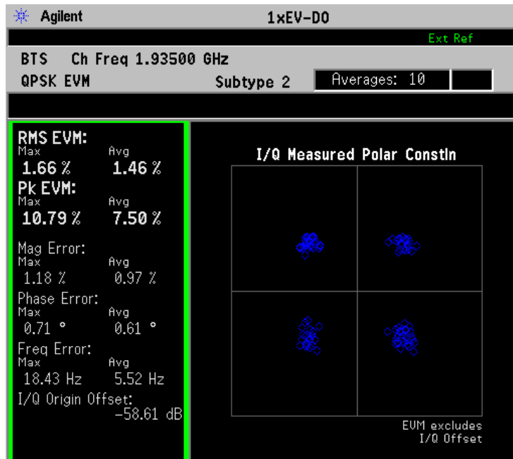
Figure 3-24 QPSK EVM Measurement - I/Q Polar Constellation View
