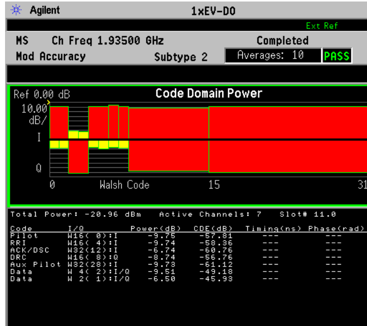
Figure 3-21 Reverse Link Modulation Accuracy - Code Domain Power View
