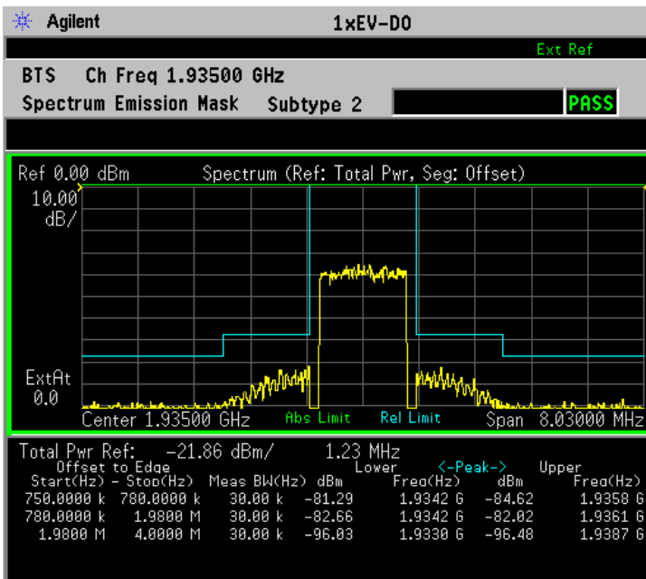
Figure 3-33 Spurious Emissions Measurement - Offset View
