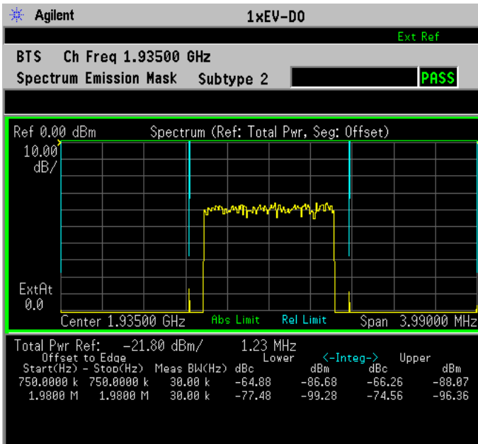
Figure 3-35 Spurious Emissions and ACP Measurement - ACP Mode View
