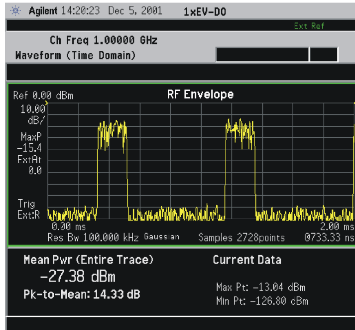
Figure 3-37 Waveform Measurement - RF Envelope (Default View)
