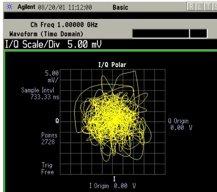
Figure 2-70 Waveform Measurement - I/Q Polar View
