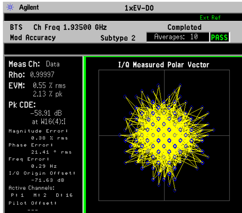
Figure 2-27 Forward Link Modulation Accuracy Measurement Result - I/Q Measured Polar Vector View
