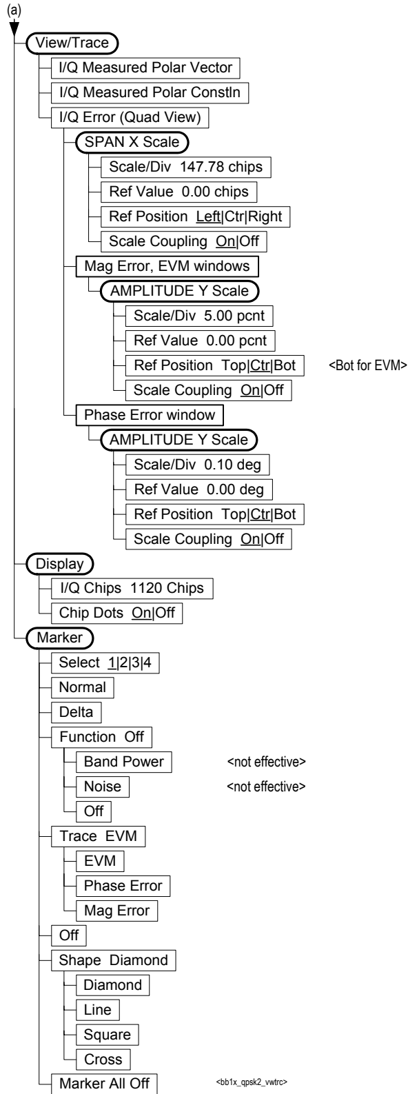
Figure 6-21 QPSK EVM Measurement Key Flow (2 of 2)
