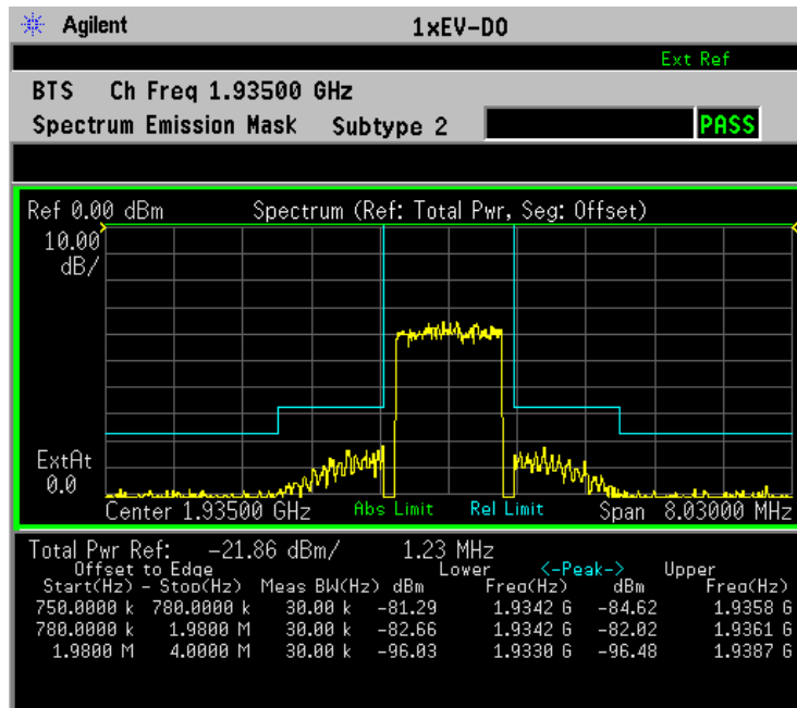
Figure 2-64 Spectrum Emission Mask Measurement Result - Offset (Default) View
