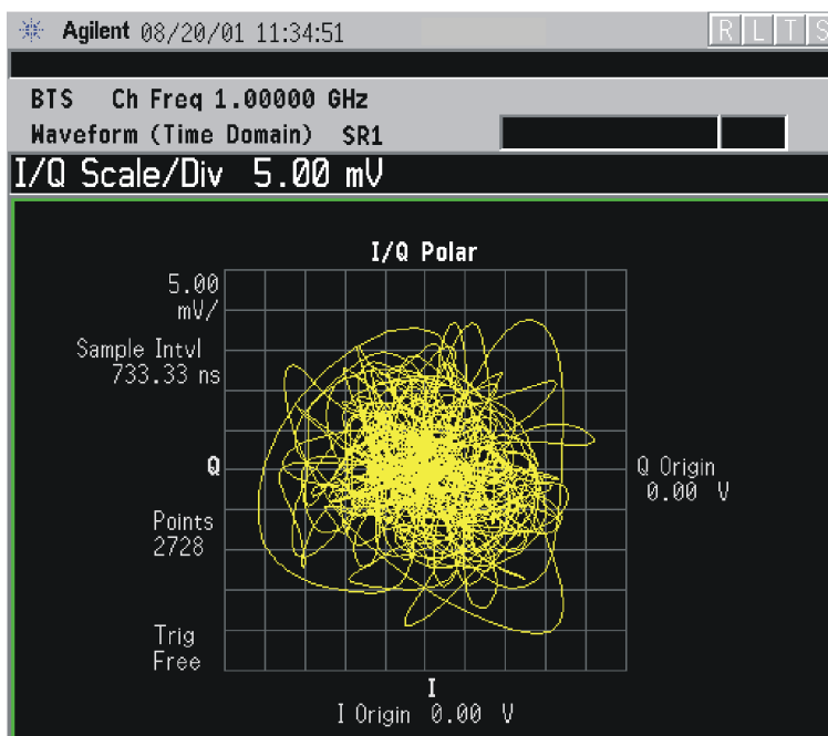
Figure 2-72 Waveform Measurement - I/Q Polar View
