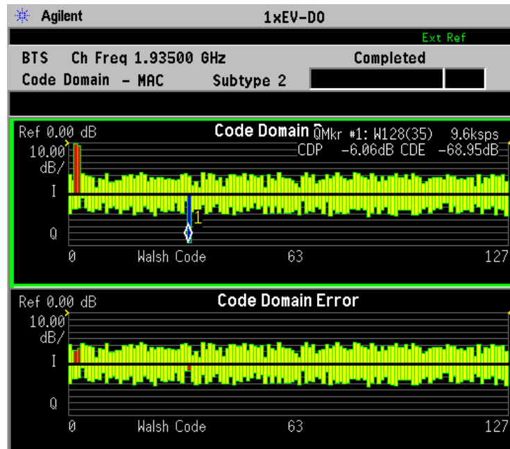
Figure 3-3 Code Domain Measurement - CDP Graph and CDE Graph View
