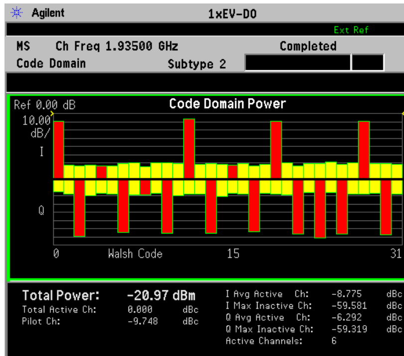
Figure 3-8 Code Domain Measurement - Power Graph and Metrics View
