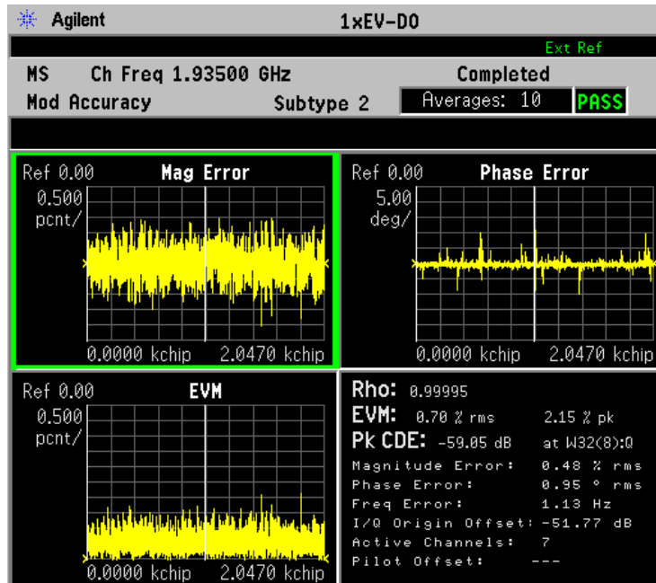
Figure 3-20 Reverse Link Modulation Accuracy - I/Q Error Quad View
