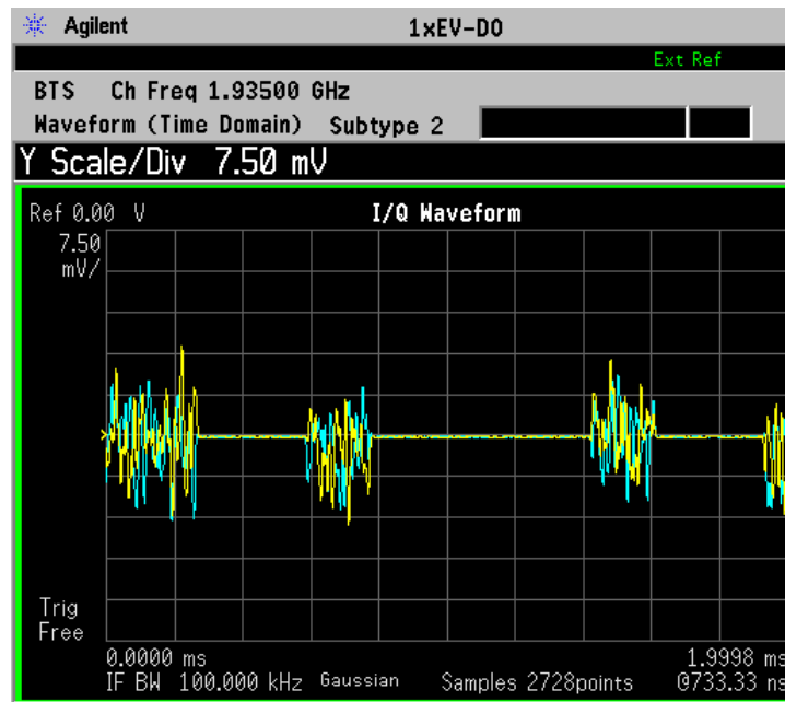
Figure 3-40 Waveform Measurement - I and Q Waveform View
