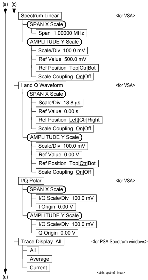
Figure 6-31 Spectrum (Freq Domain) Measurement Key Flow (3 of 4)
