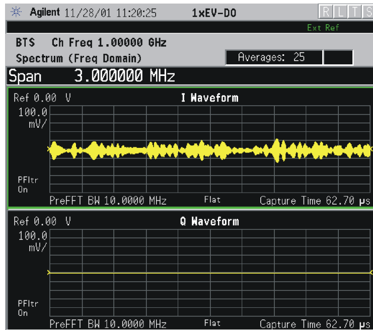
Figure 3-29 Spectrum Measurement - I and Q Waveform View (for E4406A)
