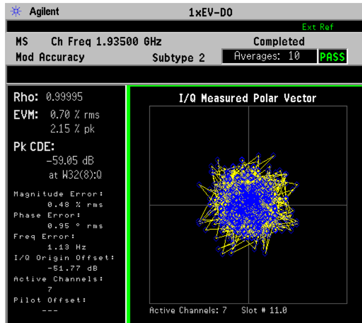
Figure 3-18 Reverse Link Modulation Accuracy - I/Q Polar Graph View
