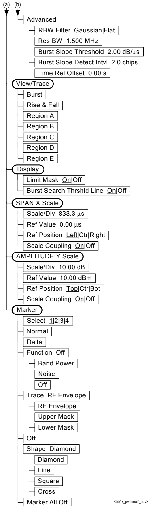
Figure 6-19 Power vs. Time Measurement Key Flow (2 of 2)
