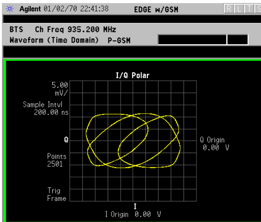
Figure 2-71 Waveform Measurement - I/Q Polar View
