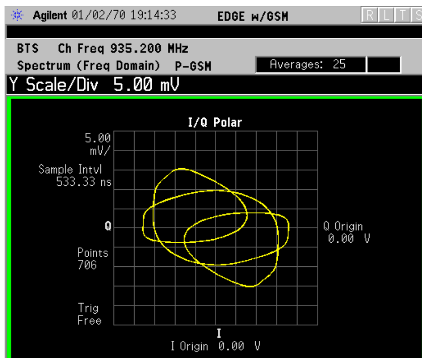
Figure 2-62 Spectrum Measurement - I/Q Polar View (for E4406A)
