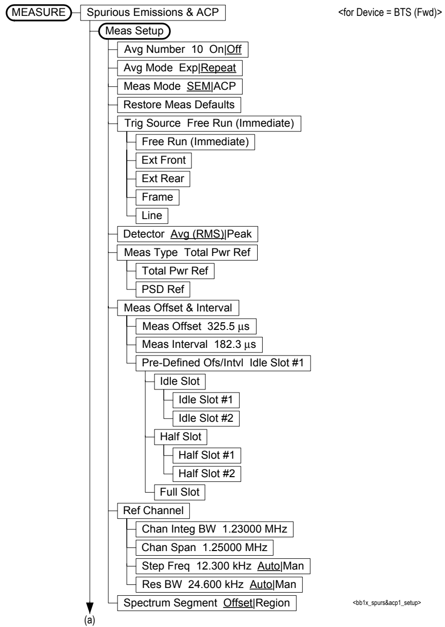
Figure 6-33 Spurious Emissions & ACP Measurement Key Flow (1 of 3)
