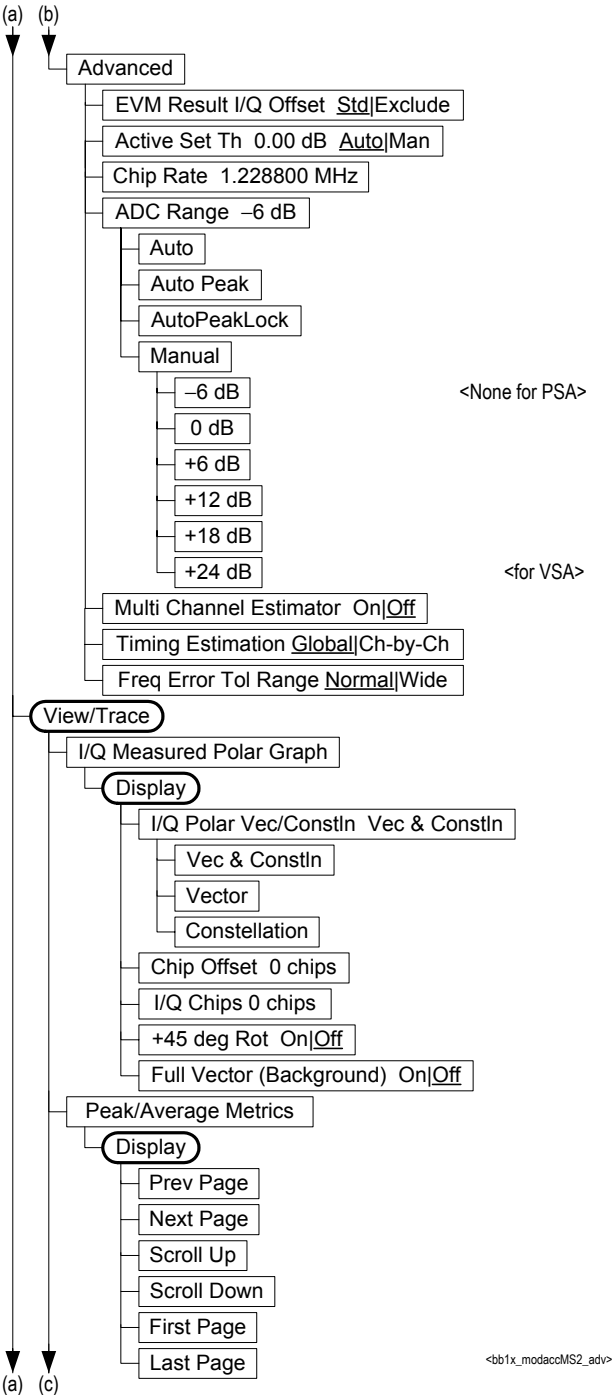
Figure 6-26 Reverse Link Mod Accuracy Measurement Key Flow (2 of 4)
