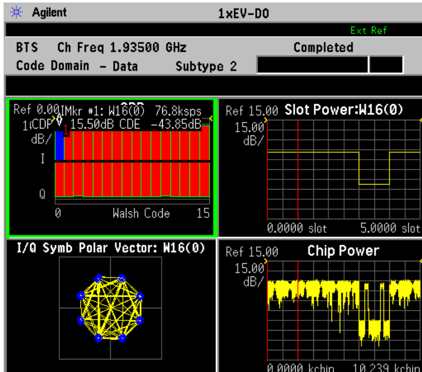
Figure 2-12 Forward Link Code Domain Results in Quad View - Data Subtype 2 with W16(0) Despread
