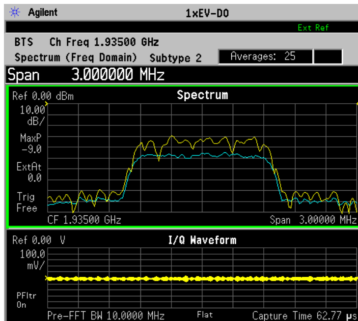
Figure 3-26 Spectrum Measurement - Spectrum and I/Q Waveform (Default View)
