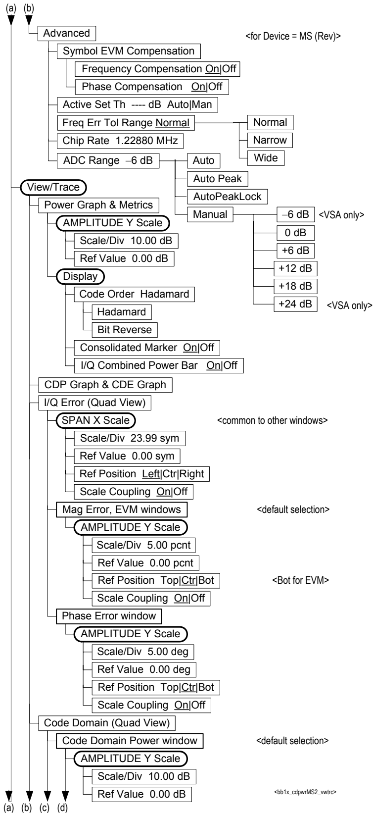
Figure 6-23 Reverse Link Code Domain Measurement Key Flow (2 of 3)
