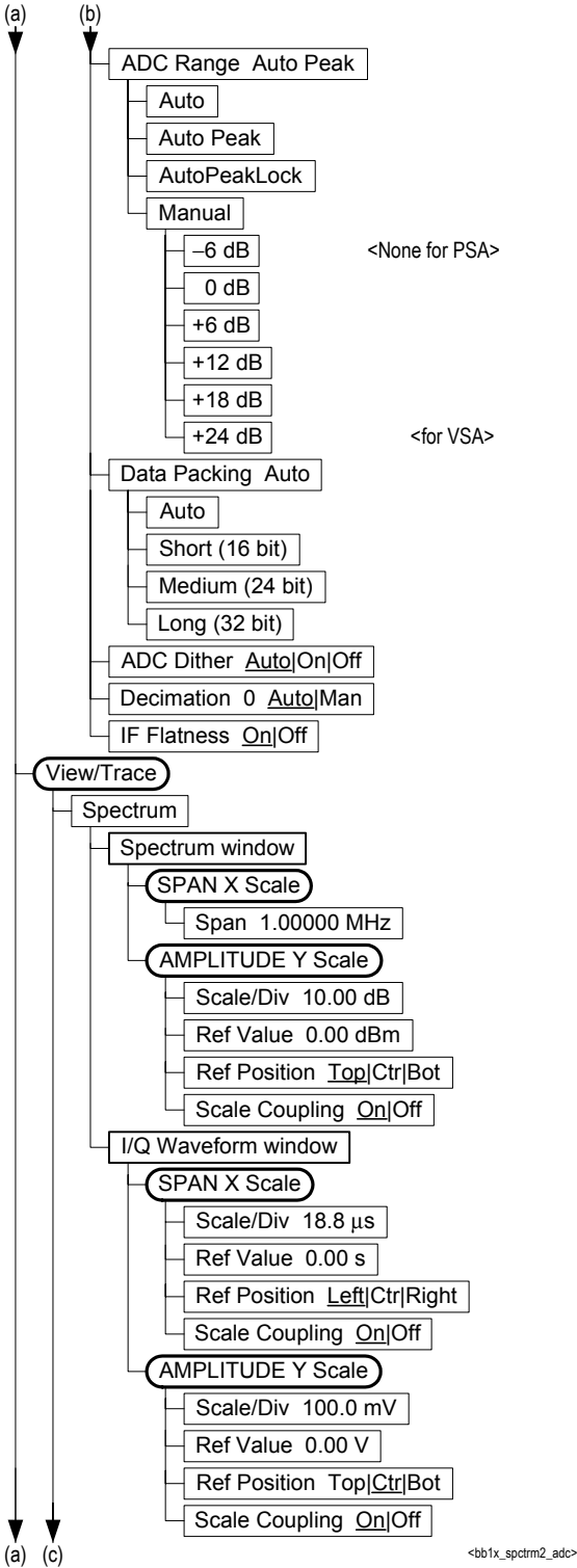
Figure 6-30 Spectrum (Freq Domain) Measurement Key Flow (2 of 4)
