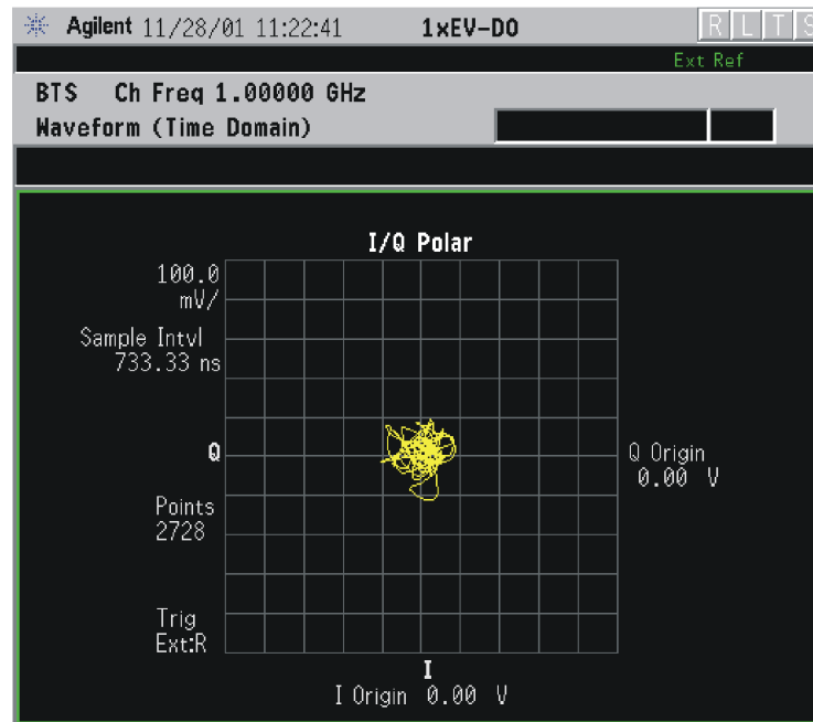
Figure 3-41 Waveform Measurement - I/Q Polar View
