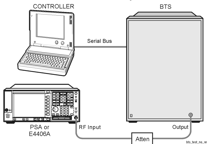
Figure 2-39 Occupied Bandwidth Measurement System
