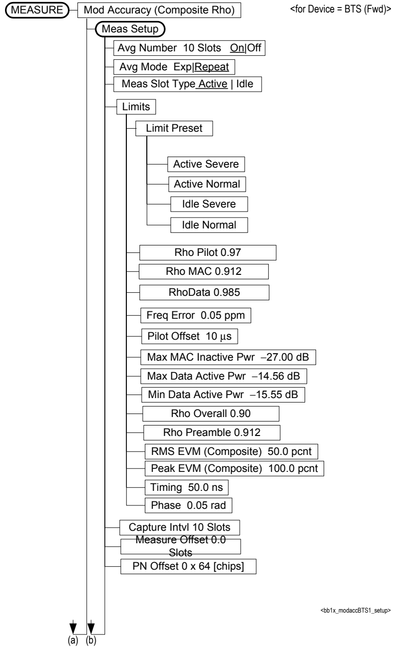
Figure 6-25 Reverse Link Mod Accuracy Measurement Key Flow (1 of 4)
