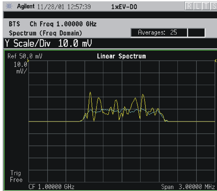
Figure 3-28 Spectrum Measurement - Linear Spectrum View (for E4406A)
