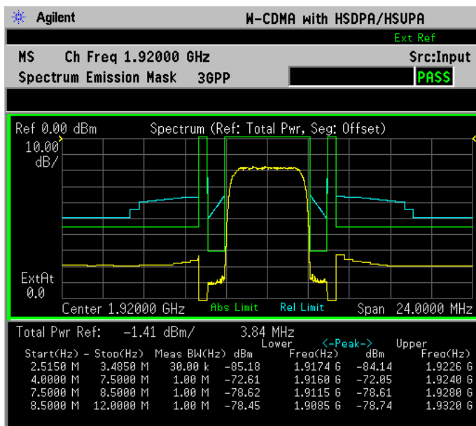
Figure 2-56 Spectrum Measurement - I and Q Waveform View (for E4406A)
