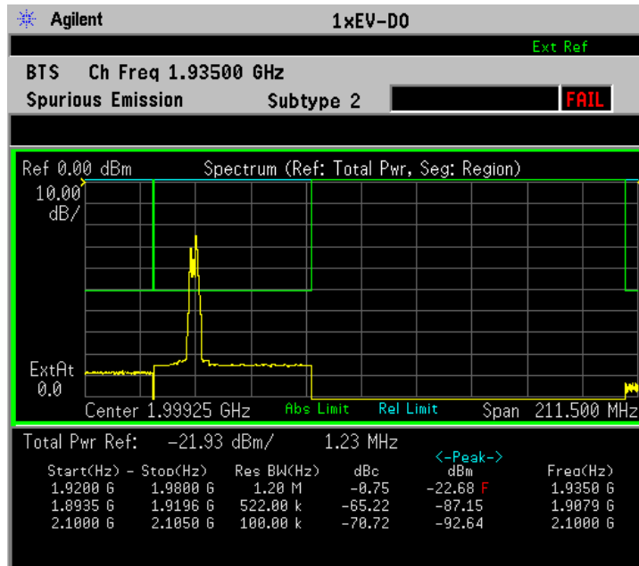
Figure 3-34 Spurious Emissions and ACP Measurement - All Regions View
