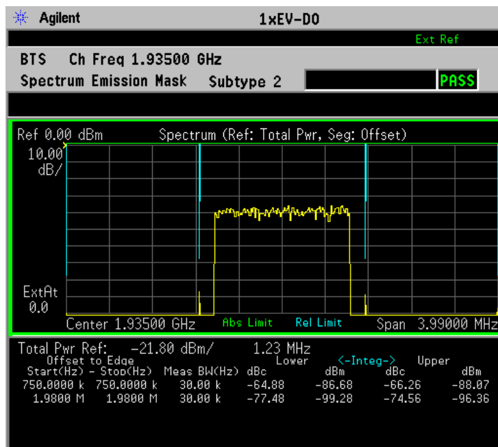
Figure 2-66 Spectrum Emission Mask Measurement Result - ACP View
