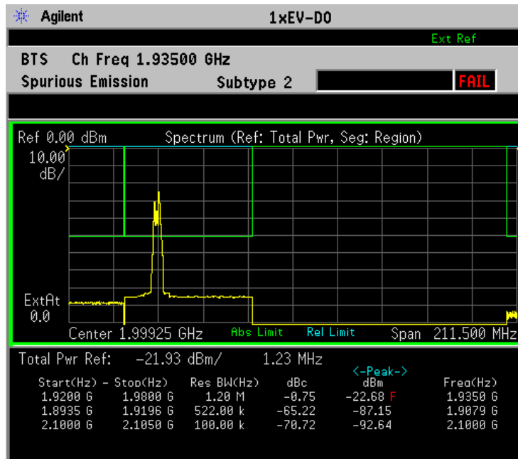
Figure 2-65 Spectrum Emission Mask Measurement Result - Region View
