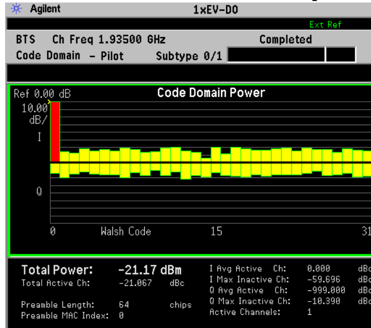
Figure 3-4 Code Domain Measurement - Power Graph & Metrics View
