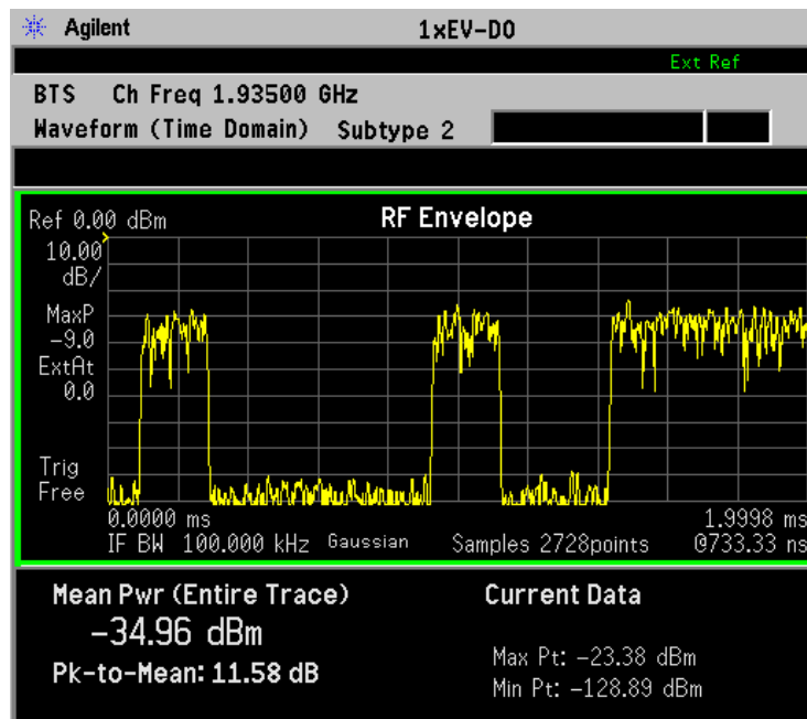
Figure 3-36 Waveform Measurement - RF Envelope (Default View)
